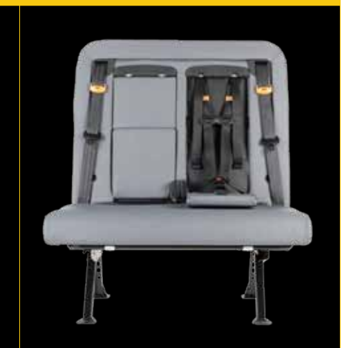
Integrated child seat with seat belt seating
